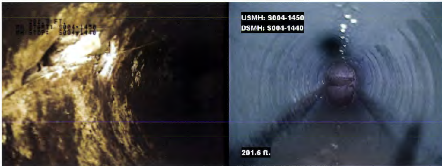
Before Hole In Pipe
